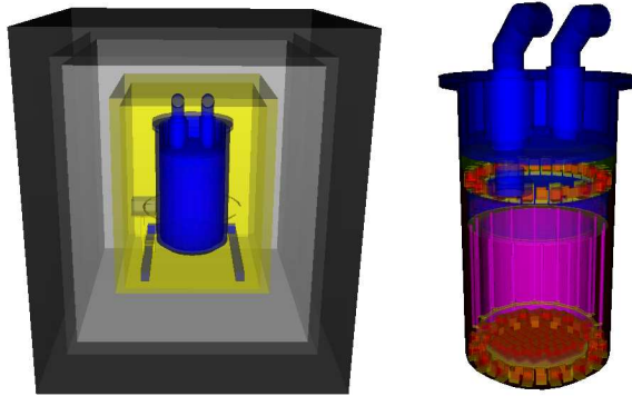
Figure 1: Left: The XENON100 detector inside its shield as it was simulated within the GEANT4 framework (the colors represent: two layers of lead - dark grey, polyethylene - light grey, and copper - yellow, water tanks are not shown; on the left side of the cryostat - lead brick for calibration with Am-Be source); Right: The closeup view of the detector (blue - stainless steel, magenta - PTFE, yellow - copper, orange - PMTs).
