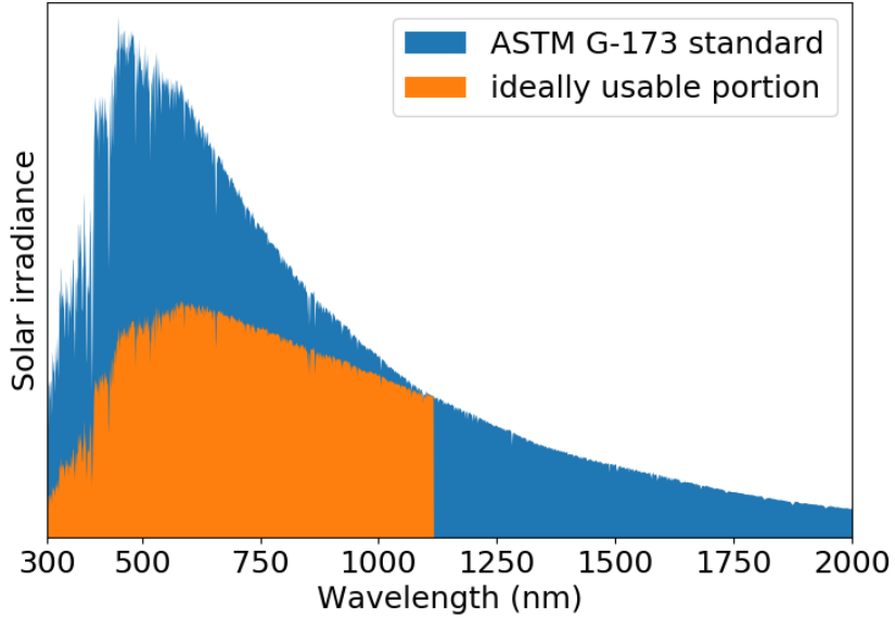
Figure 1: Solar spectrum according to the international standard ASTM G-173 (AM1.5G) and the portion of it which could be used by an idealized solar cell with E_g = 1.12 eV. Below the Si bandgap at 1100 nm a decreasingly small fraction of the spectrum can be used, while the whole tail above it remains completely unused.
