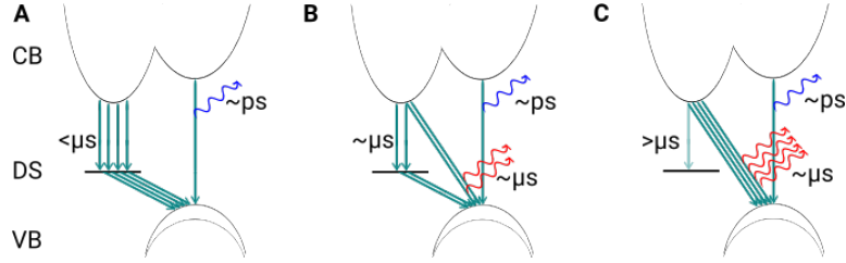
Figure 20: Schematic of decay channels at temperatures above (A), near (B) and below (C) the critical temperature T_C . CB: conduction band, VB: valence band, DS: deep state/ defect state. At high temperatures (A) the decay time constant of NR is small and most electrons follow this decay route while a small number very quickly decays via D. The contribution of D is small even though its decay time is very short because thermalisation to the CB minimum is even faster. In B the temperature has decreased to a point at which the decay times of NR and IN are comparable and PL emission from NR sets in. Finally, at low temperatures, as depicted in C, the NR decay is much slower than IN and most electrons can emit at the LT energy.
