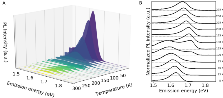
Figure 15: Results of PL measurements on \text{WSe}_2 at different temperatures. The two plots show the same data but the spectra in B have been normalized and vertically offset. A new peak starts appearing below 150 K and dominates the low temperature PL.
