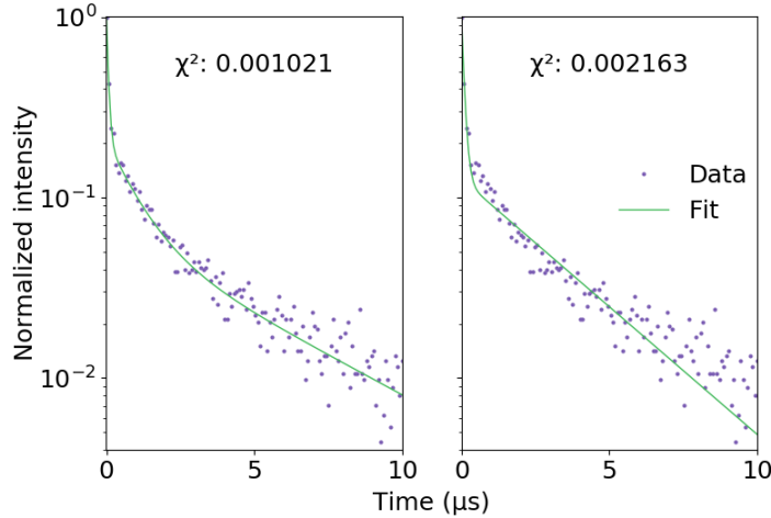
Figure 21: Comparison between a triple and a double exponential fit to the TRPL data at T = 4.2\text{ K} . The triple exponential fits the data significantly better: visually by not exhibiting a ‘kink’ at below 1\ \mu\text{s} and better match of the slope of the slow component and numerically by a halved value for \chi^2 .
